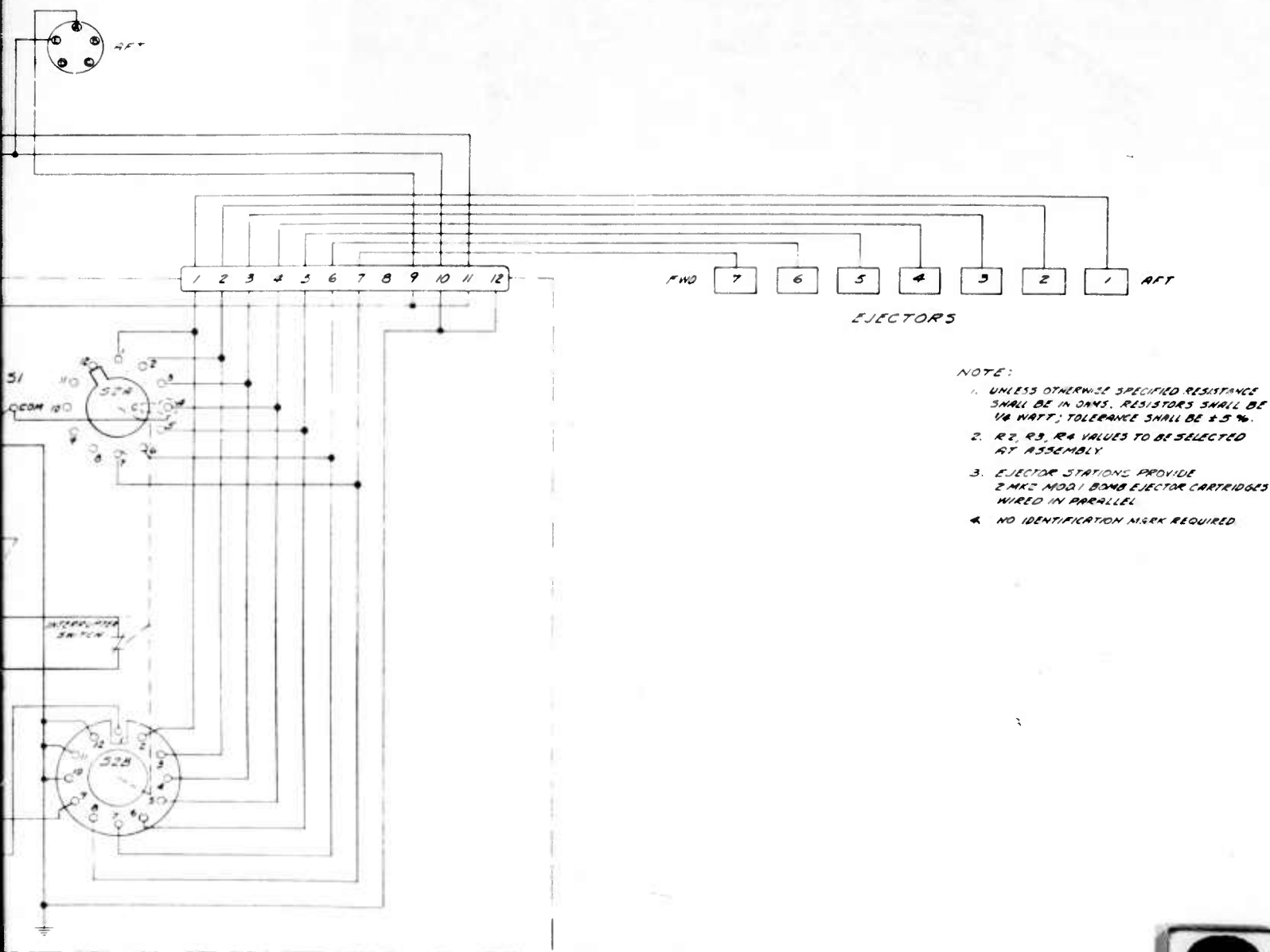
FIG. 21. Gladeye Dispenser Wiring Diagram and Intervalometer Schematic.
